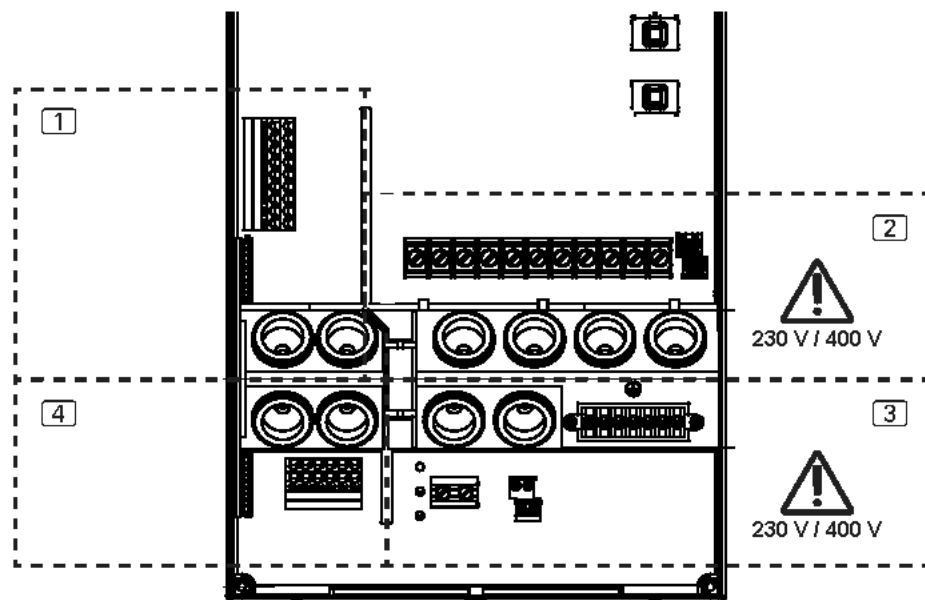
Fig. 4 Connection areas
