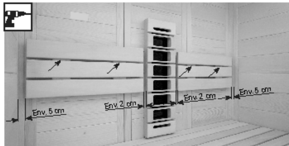
Foret de 3 mm, 4 vis 4 x 70 mm
